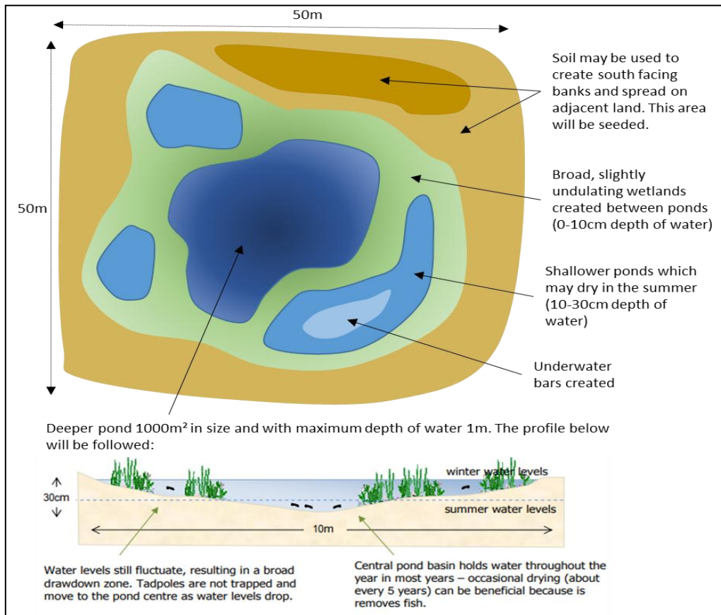
Plate 5: Suitable Pond Design
